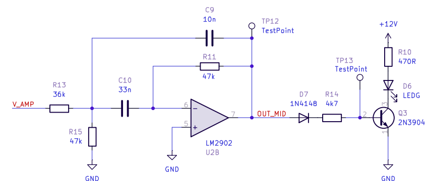
BAND-PASS FILTER
