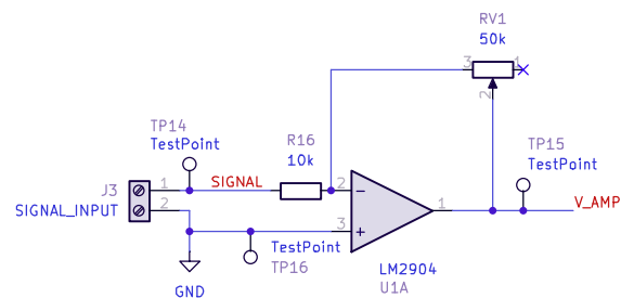
GAIN ADJ AMPLIFIER
